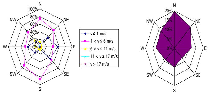
Fig.8. Wind roses charts for different sites
